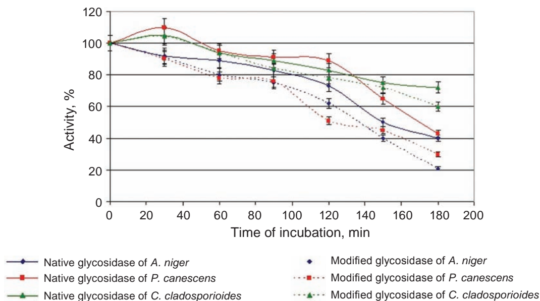
Fig. 1. Dependence of native and O-deglycosylated \alpha -galactosidase of A. niger , P. canescens , C. cladosporioides on time during thermostoinactivation (pH 5.2, 55 °C)
