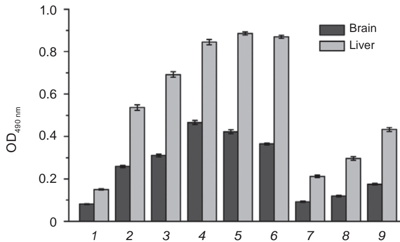
Fig. 2. Cyt c released from isolated mitochondria of the brain or liver under the effect of different Ca^{2+} doses or 0.5 \text{ mM } H_2O_2 in the presence or absence of \alpha 7 \text{ nAChR} agonist PNU282987 (30 nM): 1 – Control; 2 – 0.09 \mu\text{M } Ca^{2+} ; 3 – 0.9 \mu\text{M } Ca^{2+} ; 4 – 9 \mu\text{M } Ca^{2+} ; 5 – 45 \mu\text{M } Ca^{2+} ; 6 – H_2O_2 ; 7 – H_2O_2 + PNU ; 8 – 0.09 \mu\text{M } Ca^{2+} + PNU ; 9 – 9 \mu\text{M } Ca^{2+} + PNU . Each column corresponds to OD_{490 \text{ nm}} mean \pm S.E. ( n = 3 ) defined by sandwich ELISA
