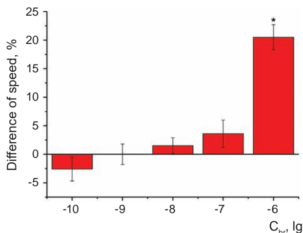
Fig. 2. Influence of des-arg 9 -bradykinin acetate on Vn smooth muscle contraction of rats stomachs (* P < 0.05 ). (Comparison with amplitude (mN) and maximal normalized rate (Vn) of contraction upon impact of bradykinin only (line "0"))
