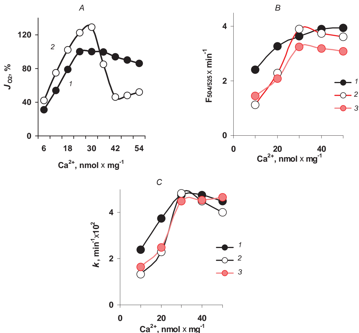
Fig. 3. The influence of MPTP opening on the oxygen consumption (A) and ROS formation (B-C) in the rat brain mitochondria. A: The influence of MPTP opening on the rate of respiration. B-C: The influence of MPTP opening on the rate of ROS formation under steady-state (B) and non-equilibrium (C) conditions. MPTP was blocked by the addition of cyclosporine A (A-C, 1). Incubation medium: 320 mM sucrose, 1 mM \text{KH}_2\text{PO}_4 , 5 mM of sodium succinate, 5 mM Tris-HCl buffer (pH 7.4). Cyclosporine A (A, 1; B-C, 1,3) and A-23187 (B-C, 3) were added at 1\mu\text{M} ; \text{CaCl}_2 in \text{nmol}\cdot\text{mg}^{-1} protein was added as shown on the abscissa (A-C). M\pm S.D. , n = 6 , P < 0.05 relative to control (A-C, 1).
