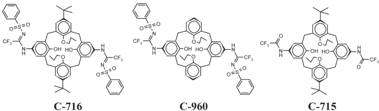
Fig. 4. Tert -butyl-calixarenesulfonylamidide C-716 and its tert -butyl depleted (C-960) and thioacetamide (C-715) analogs
